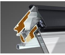
5 Excellent insulation • expanded polystyrene • colour: grey charcoal • thermally modified timber
